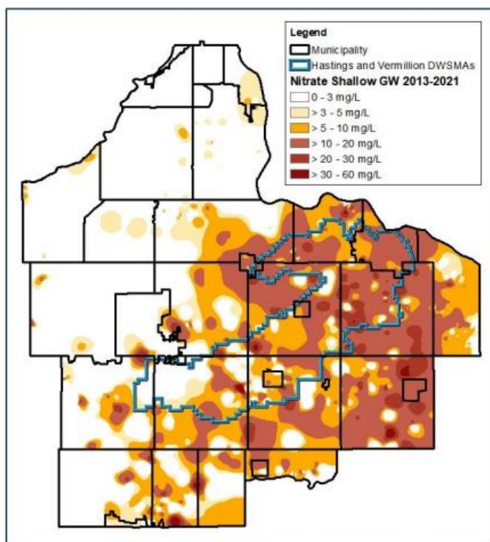
Figure 3: Interpolation of shallow groundwater nitrate concentrations (in mg/L \text{NO}_3\text{-N} ), adapted from Dakota County ACRE Plan (Dakota County, 2022)
