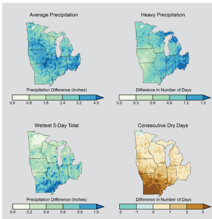
Figure 4: Projected precipitation change for the middle of the current century (2041-2070) relative to last century (1971-2000) in Midwest. (National Climate Assessment, 2014)
