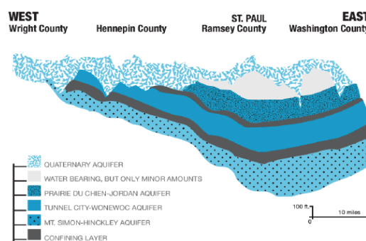
Figure 2: Regionally significant aquifers
